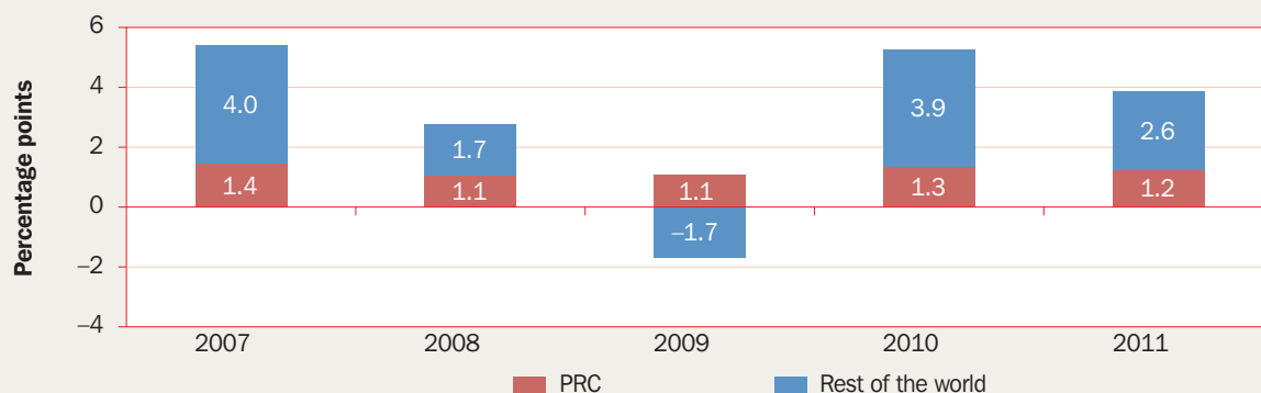
Figure 1.2 Contribution of the PRC to global growth, 2007–2011
